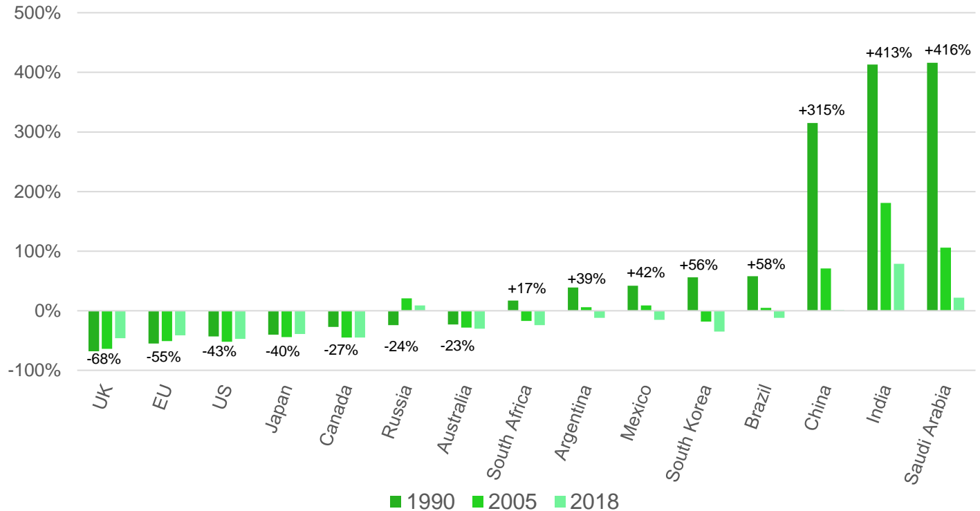
G20 countries' emissions pledges by 2030 relative to 1990, 2005 and 2018 levels (% number = from 1990 level)
